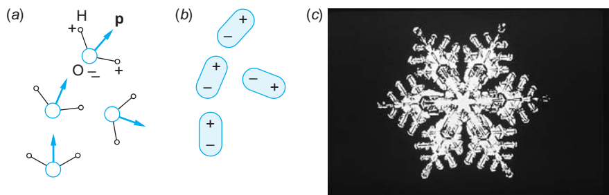
FIGURE 9-19 (a) Schematic of four \text{H}_2\text{O} molecules. The water molecules' permanent dipole moments are shown by the vectors \mathbf{p} . (b) The four polar water molecules represented as electric dipoles. Notice that the attractive dipole-dipole force tends to align the dipoles so that the nearest neighbors of each charge are charges of the opposite sign. (c) A snowflake—one result of dipole-dipole bonding.
